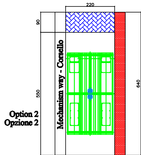
Car pallet layout in single bay Layout posti auto in singola baia
